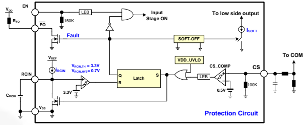
Figure 42. Over-Current Protection
