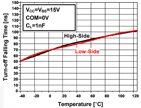
Figure 11. Turn-Off Falling Time vs. Temp.
